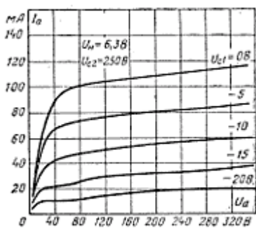
Plate curves
